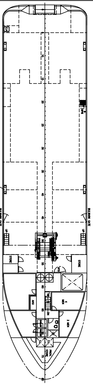
MAIN DECK
