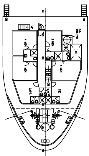
FORECASTLE DECK
